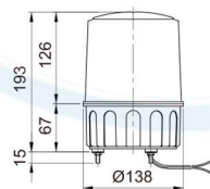
S150U/ S150ULR
