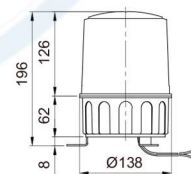
S150U-FT/ S150ULR-FT
